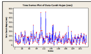
Figure 1. Rainfall Data of Mamasa Station year 1990 to 2012
