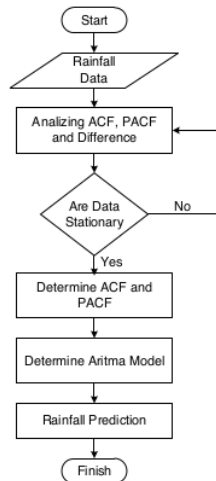
Figure 4. Flow chart prediction with ARIMA models
