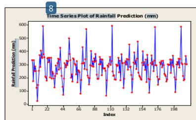
Figure 5. Results predicted rainfall in 2013 and 2030 Mamasa station
