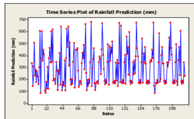
Figure 7. Results predicted rainfall in 2013 and 2030 Lembang station
