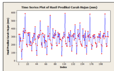
Figure 6. Results predicted rainfall in 2013 and 2030 Sumarong station
