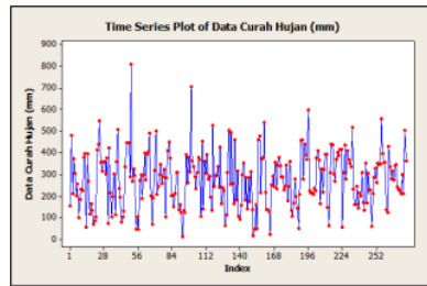
Figure2. Rainfall Data of Sumarorong Station year 2009 to 2012
