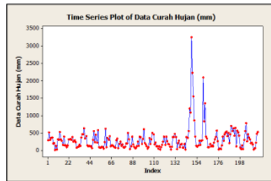
Figure3. Rainfall Data of Lembang Station year 2009 to 2012
